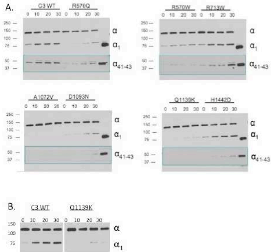
Figure 2.6. Cofactor assays utilizing the mutant C3 proteins. C3 preparations were incubated for 0 to 30 min at 37°C with FI and a cofactor protein (MCP in panel A, FH in B). The time zero control is prior to the addition of FI. The last lane is a purified iC3b control (10 ng/lane). Samples were reduced and analyzed by Western blotting using either chicken anti- human C3 or goat anti-human C3 (insets) followed by an HRP-linked secondary Ab. Cofactor activity is assessed by a reduction in the quantity of the \alpha -chain and appearance of the \alpha_1 and \alpha_{43-41} kDa cleavage fragments. Data are representative of 5 experiments. The chicken Ab recognizes poorly the \beta -chain, while the goat Ab stains more efficiently the \alpha_{41} and \alpha_{43} fragments.
